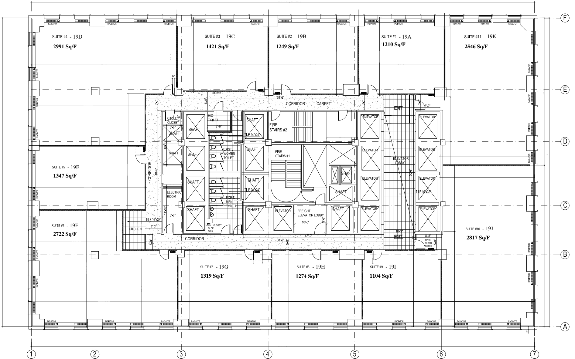
INTERIOR PLAN 19 FLOOR
